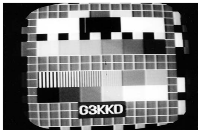
70cm, 1.25MHz bandwidth, off air pictures
