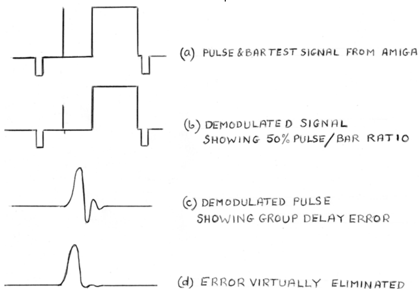
Fig 8 GROUP DELAY WAVEFORMS 10-8-01
